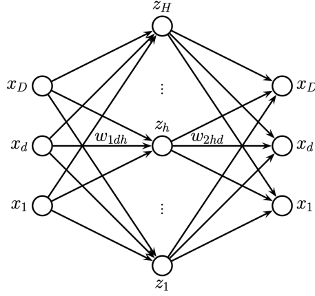
Figure 1: An autoencoder with one hidden layer MLP
